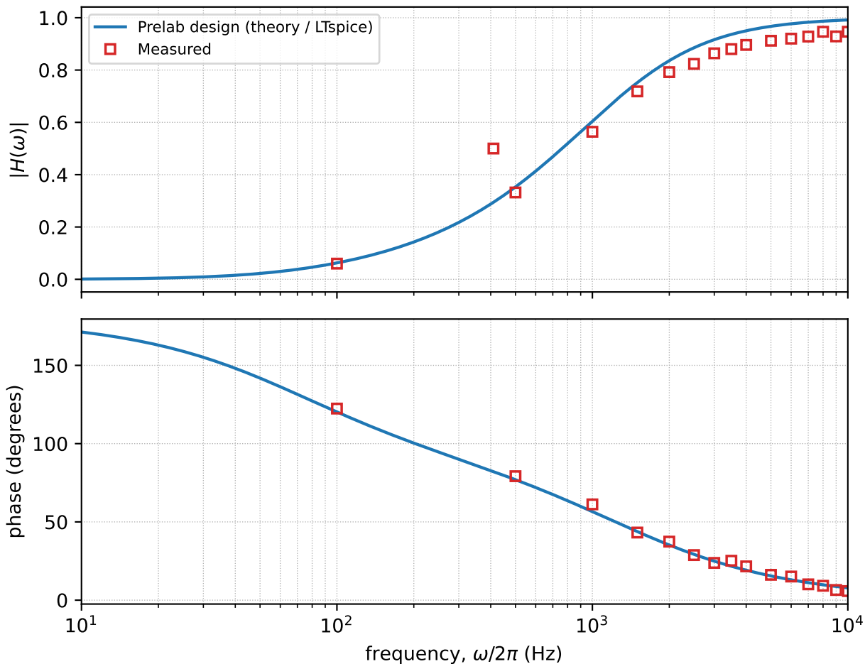
High-pass Sallen-Key: magnitude and phase response
